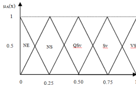
Figure 2. TFN of linguistic preference
